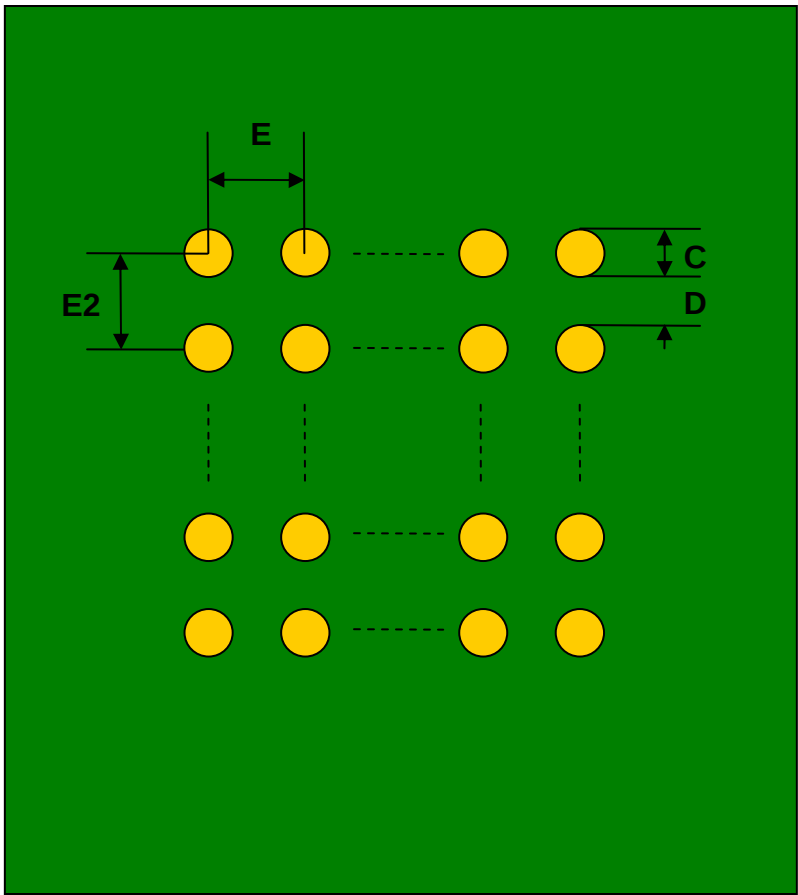
Top View (SMT Footprint)
