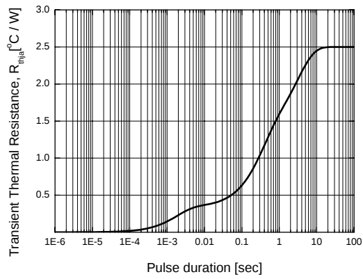
Figure 7. Thermal Resistance
