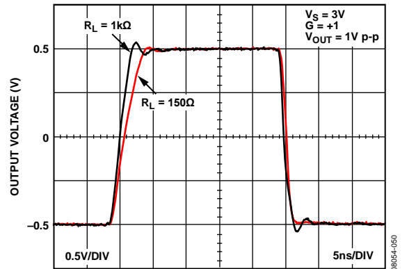
Figure 36. Large-Signal Step Response, V_S = 3V , G = +1
