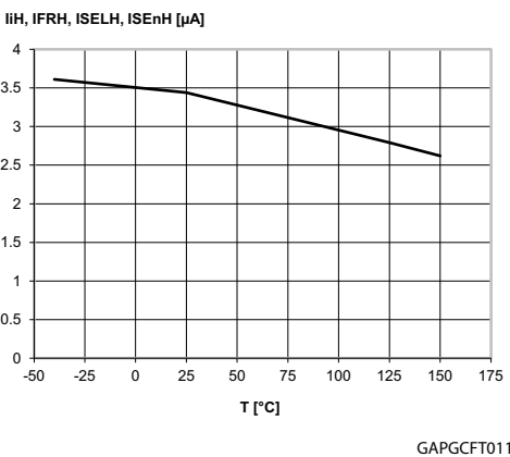
Figure 20. High level logic input current
