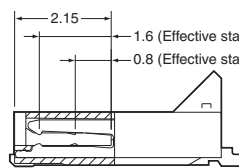
Cross-section diagram: X-X
