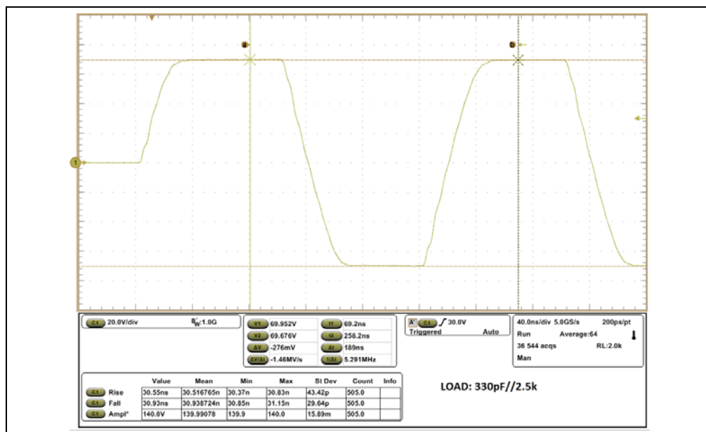
FIGURE C-1: 5 MHz V_{PP}/V_{NN} = \pm 80V Load: 330 pF//2.5K.
