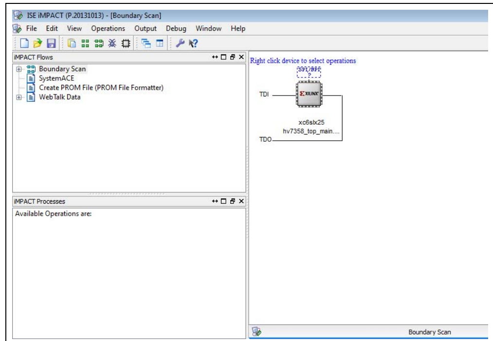
FIGURE 4-5: SPI/BPI Window.
