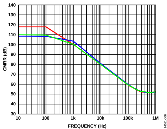
Figure 6. CMRR vs. Frequency
