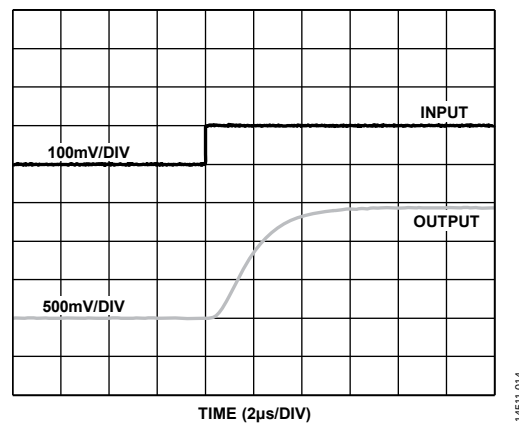
Figure 14. Rise Time
