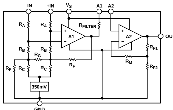
Figure 23. Simplified Schematic
