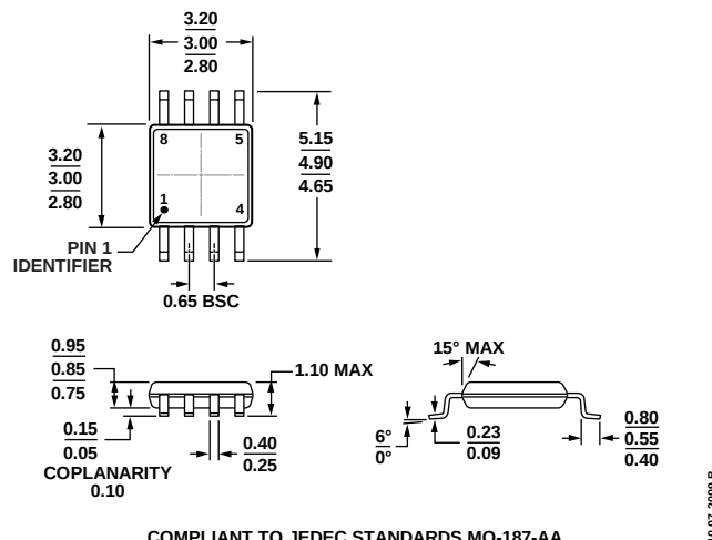
Figure 37. 8-Lead Mini Small Outline Package [MSOP] (RM-8)
