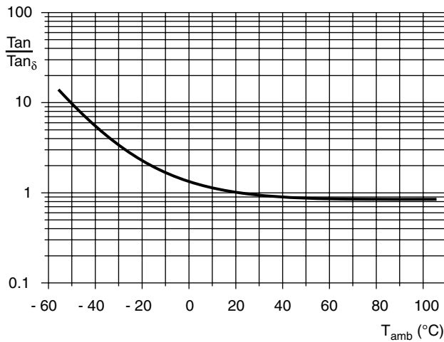
Fig.9 Typical multiplier of dissipation factor \tan \delta as a function of temperature at 20 at 100 Hz \tan \delta_0 = typical \tan \delta at 20 °C, 100 Hz
