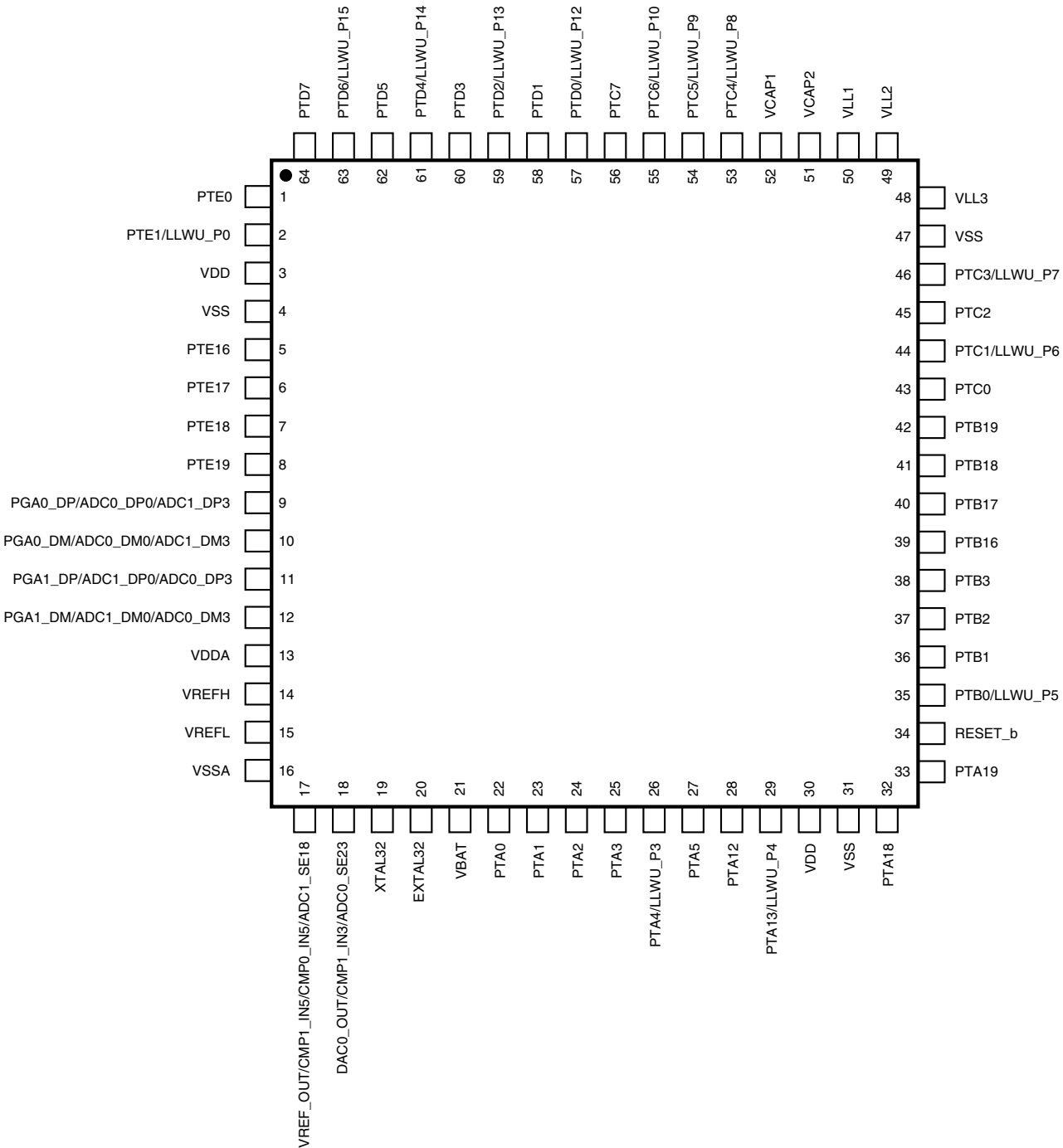
Figure 27. K30 64 LQFP/QFN Pinout Diagram
