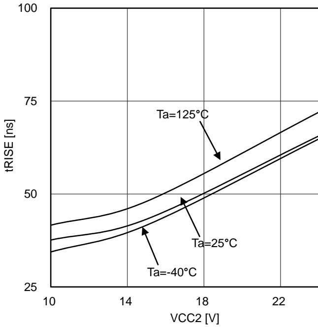
Figure 29. Rise Time vs Output Side Supply Voltage (10nF between OUT-GND2)
