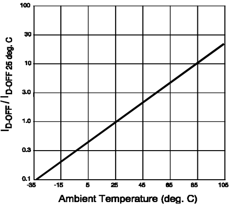
Figure 4. Typical Normalized Off-State Leakage
