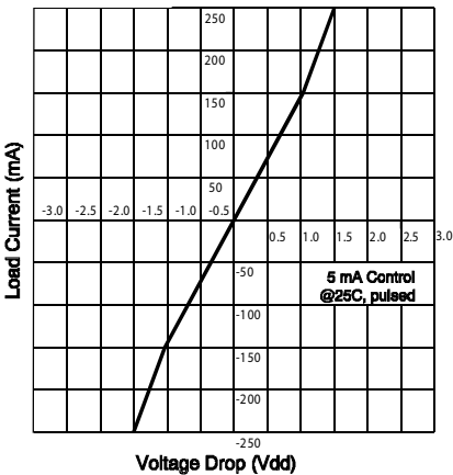
Figure 2. Linearity Characteristics
