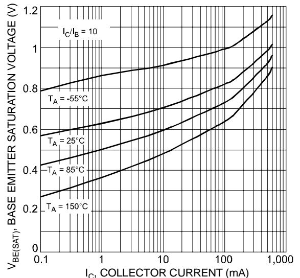
Fig. 5 Typical Base Emitter Saturation Voltage vs. Collector Current (2222A)
