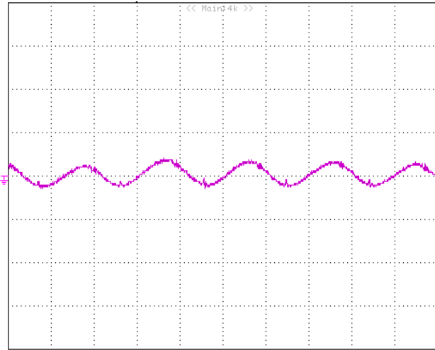
Figure 12: Input reflected ripple current, i_s , through a 12\mu\text{H} source inductor at nominal input voltage and rated load current ( 20\text{mV/div} , 2\mu\text{s/div} ).
