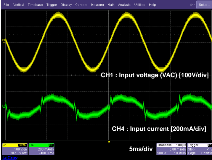
Figure6. Input waveform
