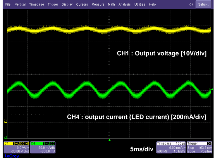
Figure7. Output waveform
