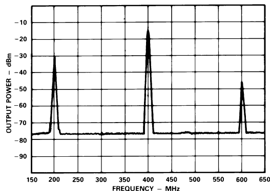
Figure 15. Output Spectrum for Configuration of Figure 14
