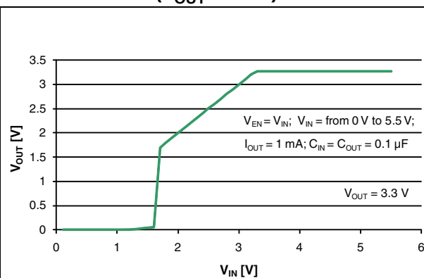
Figure 10. Output voltage vs. input voltage ( V_{OUT} = 3.3\text{ V} )
