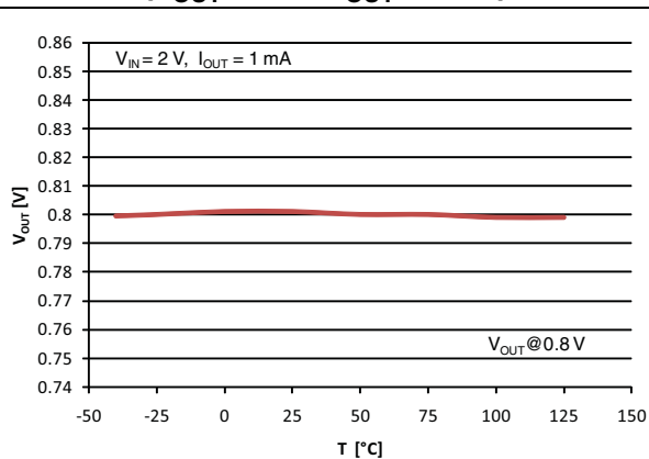
Figure 6. Output voltage vs. temperature ( V_{OUT} = 0.8\text{ V} , I_{OUT} = 1\text{ mA} )
