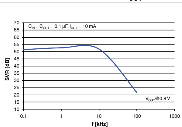
Figure 12. SVR vs. frequency (C OUT = 0.1 μF)
