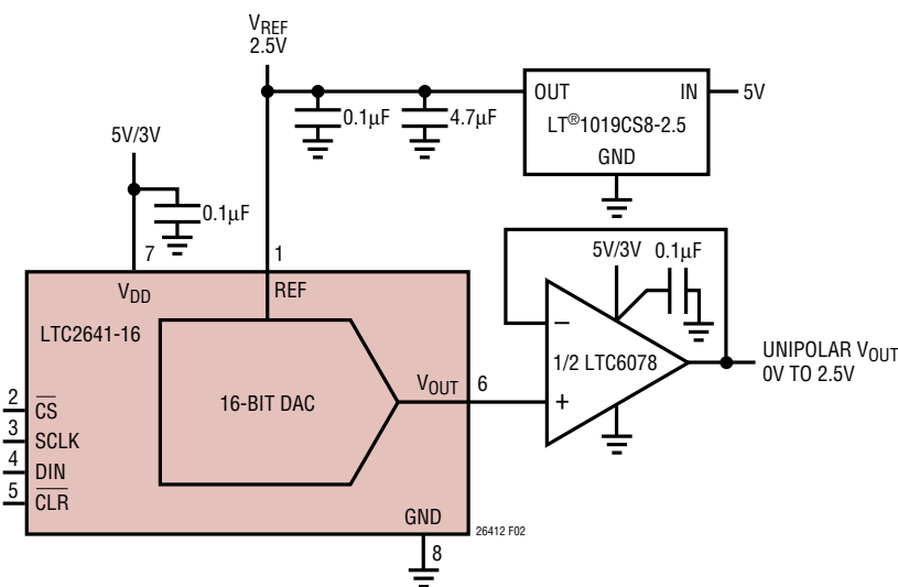
Figure 2. 16-Bit Unipolar Output (LTC2641-16) Unipolar V_{OUT} = 0V to V_{REF}
