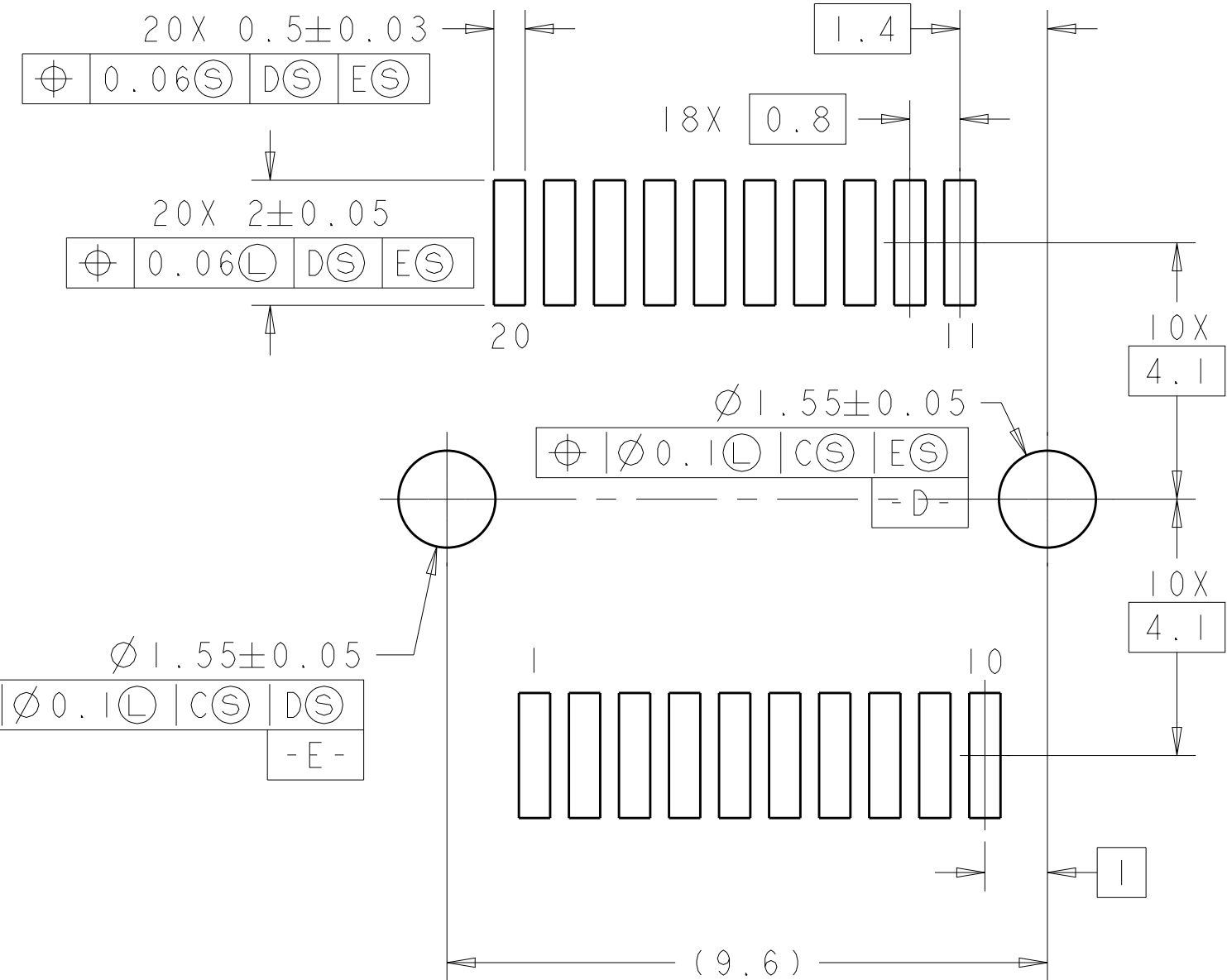
DETAIL F RECOMMENDED PT CONNECTOR LAYOUT 4X INDIVIDUALLY SCALE 10:1
