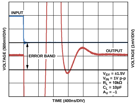
Figure 55. Negative Settling Time to 0.1%
