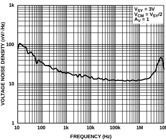
Figure 56. Voltage Noise Density vs. Frequency
