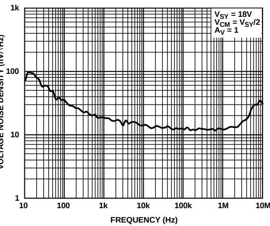
Figure 59. Voltage Noise Density vs. Frequency
