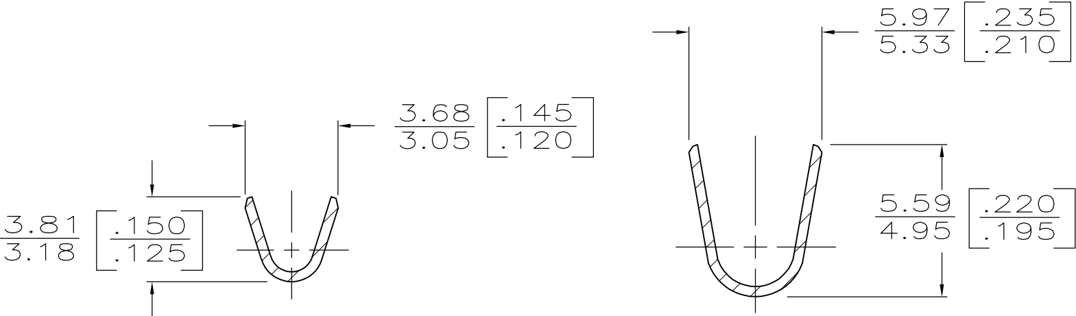
SECTION B-B
