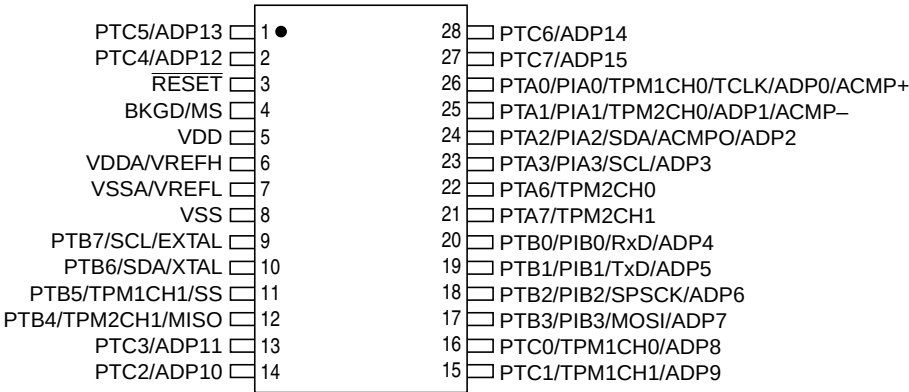
Figure 2-1. 28-Pin TSSOP
