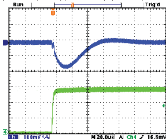
Step Load Transient Response (Vin=12V, Vout=5V, Cload=10x10µF X5R 0805 ceramic, plus 1x470µF, 7mΩ POSCAP, total 570µF, Iout=0A to 1.5A) Top trace=Vout, Bottom trace=Iout
