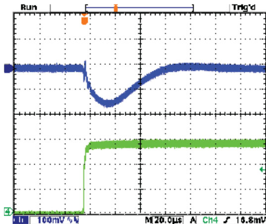
Step Load Transient Response (Vin=12V, Vout=3.3V, Cload=10x10µF X5R 0805 ceramic, plus 1x470µF, 7mΩ POSCAP, total 570µF, Iout=0A to 1.5A) Top trace=Vout, Bottom trace=Iout
