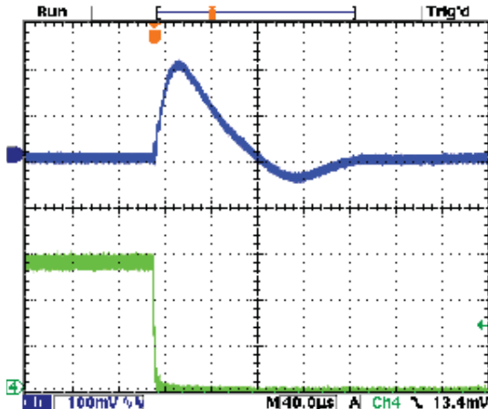
Step Load Transient Response (Vin=4.5V, Vout=1.8V, Load=10x10µF X5R 0805 ceramic, plus 1x470µF, 7mΩ POSCAP, total 570µF, Iout=1.5A to 0A) Top trace=Vout, Bottom trace=Iout
