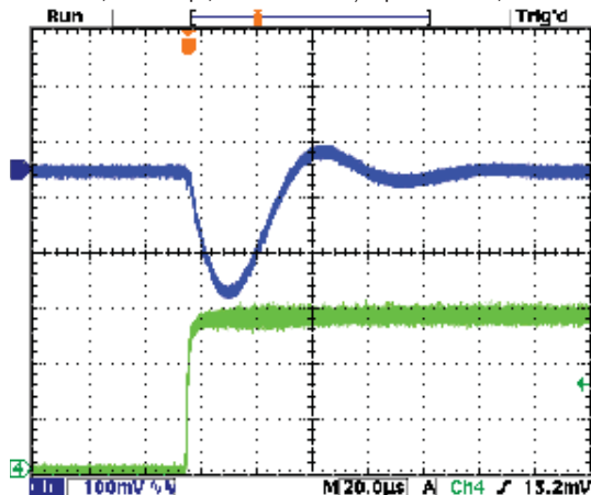
Step Load Transient Response (Vin=7.5V, Vout=5V, Cload=10x10µF X5R 0805 ceramic, plus 1x470µF, 7mΩ POSCAP, total 570µF, Iout=0A to 1.5A) Top trace=Vout, Bottom trace=Iout
