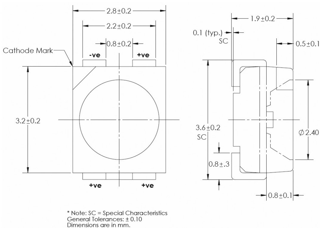
Figure 8. Mechanical dimensions for SignalSure 150.
