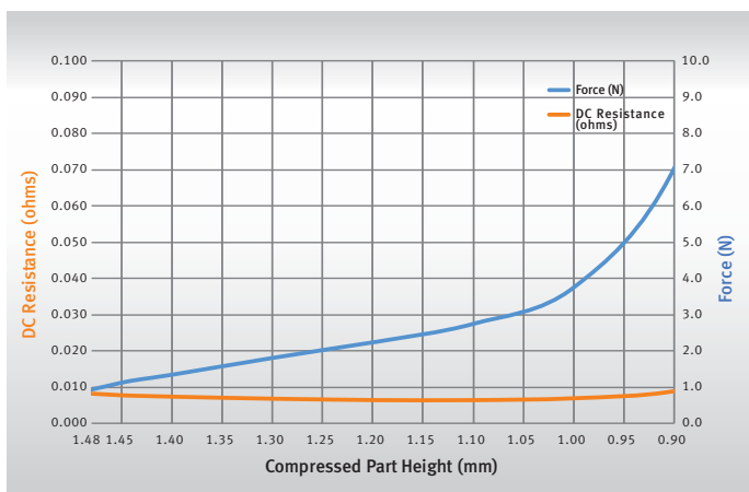
FIGURE 4: FORCE DISPLACEMENT RESISTANCE FOR 25SMT-6110-01
