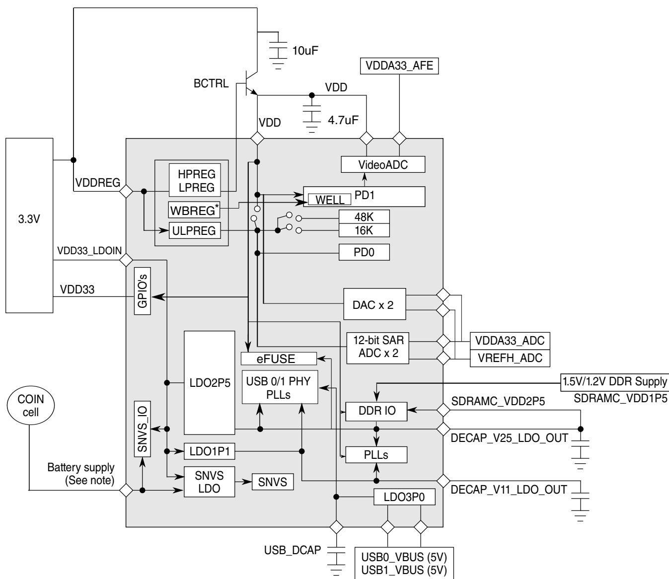
Figure 4. Power supply
