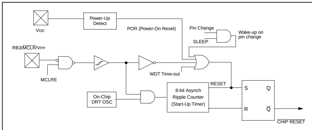
FIGURE 7-9: TIME-OUT SEQUENCE ON POWER-UP ( \overline{\text{MCLR}} PULLED LOW)
