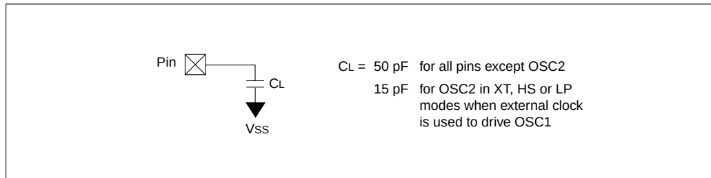
FIGURE 10-1: LOAD CONDITIONS - PIC16C505
