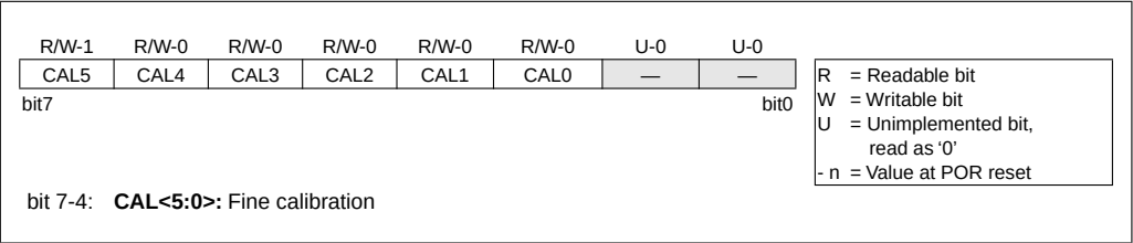
FIGURE 4-5: OSCCAL REGISTER (ADDRESS 05h)PIC16C505
