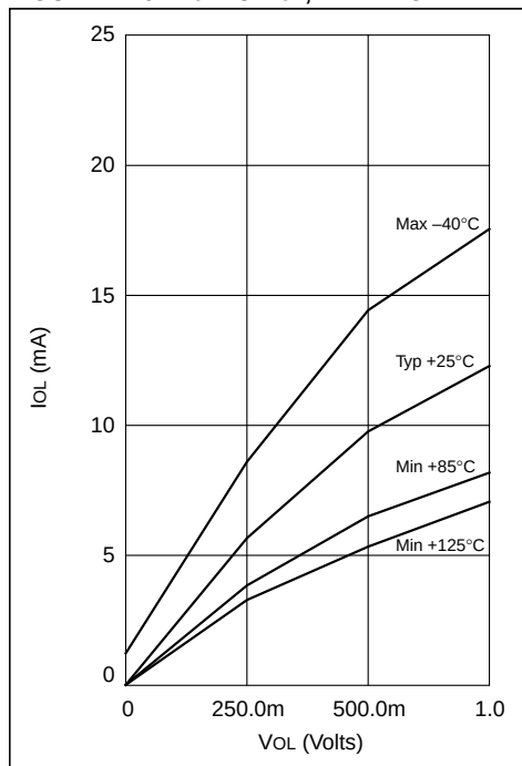
FIGURE 11-10: I_{OL} vs. V_{OL} , V_{DD} = 5.5\text{ V}
