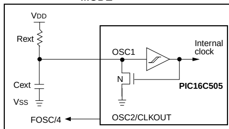
FIGURE 7-6: EXTERNAL RC OSCILLATOR MODE
