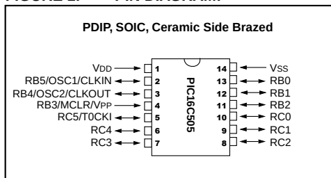
FIGURE 1: PIN DIAGRAM:
