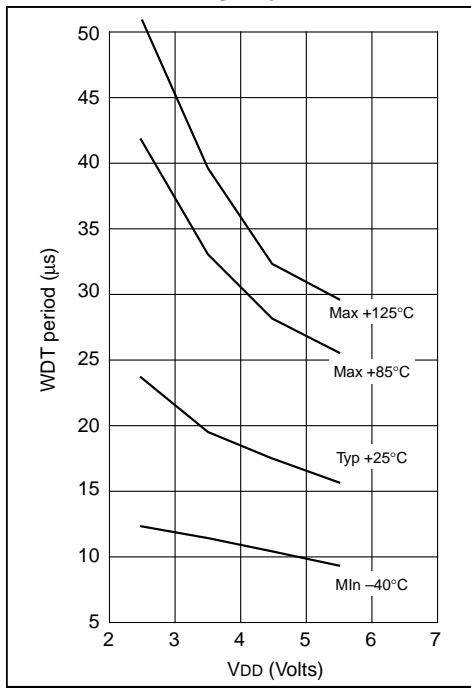
FIGURE 11-5: WDT TIMER TIME-OUT PERIOD vs. VDD
