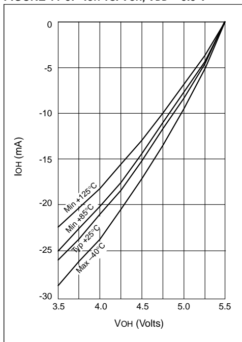
FIGURE 11-8: I_{OH} vs. V_{OH} , V_{DD} = 5.5 V
