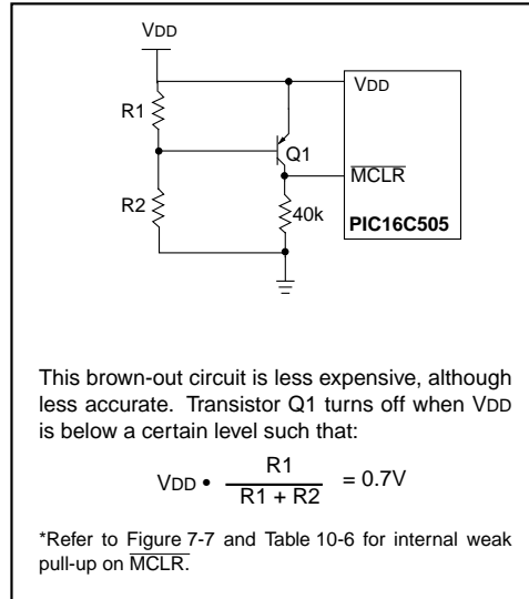
FIGURE 7-14: BROWN-OUT PROTECTION CIRCUIT 2
