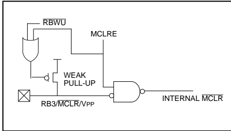
FIGURE 7-7: MCLR SELECT
