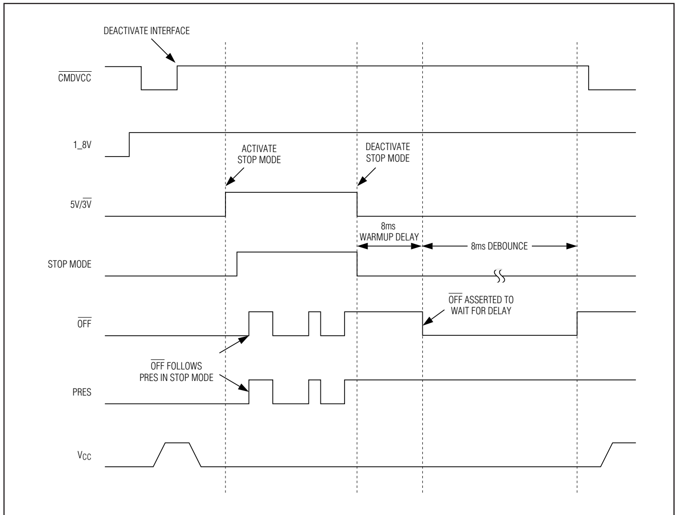
Figure 8. Stop-Mode Sequence
