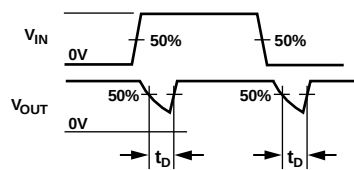
Figure 18. Break-Before-Make Time Delay, t_D
