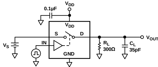
Figure 17. Switching Times
