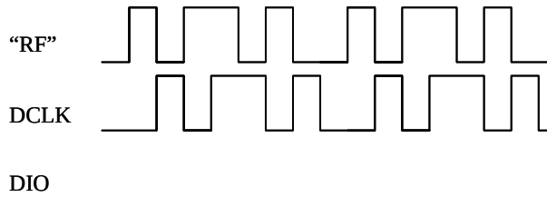
Figure 11. Transparent Asynchronous UART mode ( SEP\_DI\_DO = 1 )
