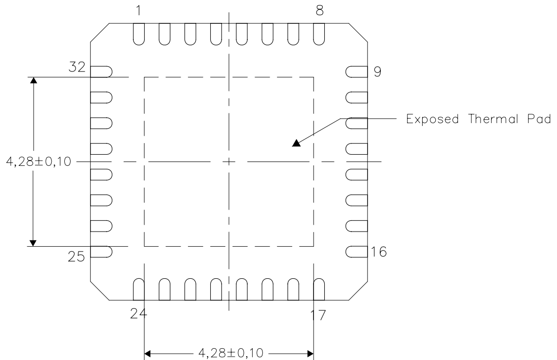
Bottom View
