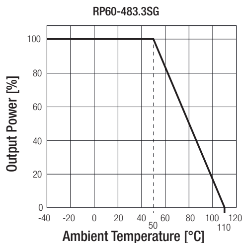
Derating Graph (11)
