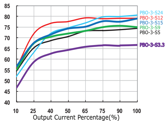
Efficiency Curve (Efficiency vs. Load Current)
