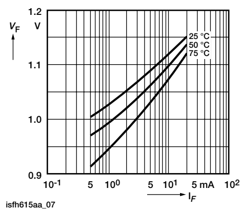
Fig. 7 - Diode Forward Voltage (Typ.) vs. Forward Current
