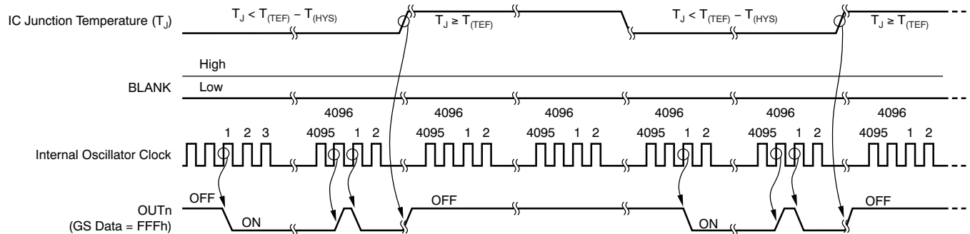
Figure 22. TSD Operation
