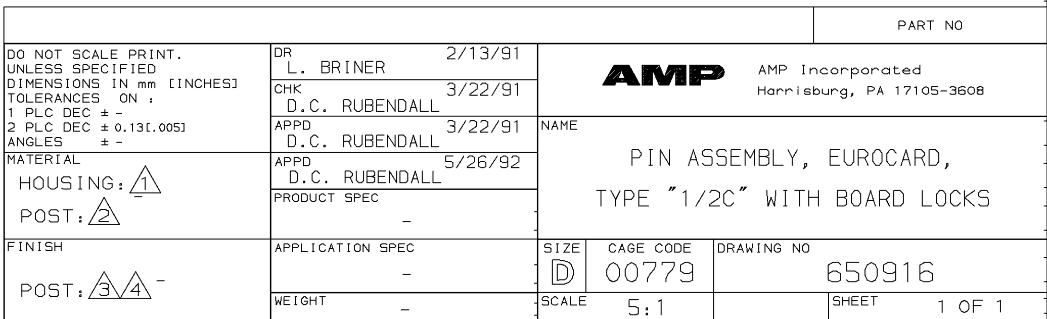
OBSOLETE 3 1-16 X X X 48 650916-9 4 1-16 X X X 48 650916-5 NOTES POSITIONS LOADED C B A NO. OF LOADED POSITION ASSY PART NUMBER ROWS LOADED
