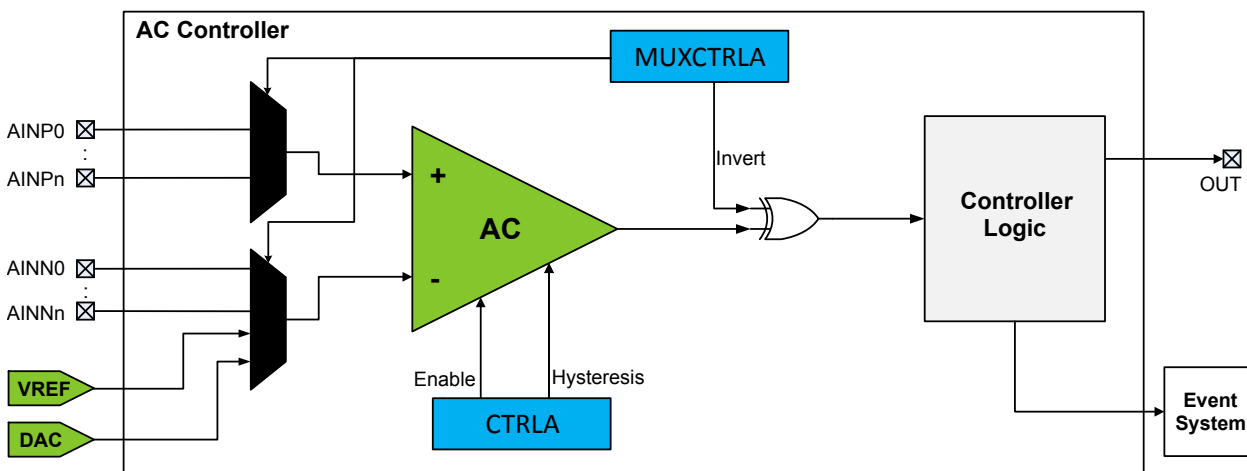
Figure 29-1. Analog Comparator
