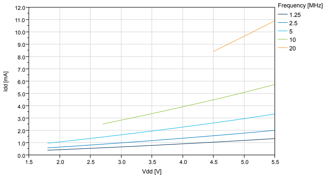
Figure 35-4. Active Supply Current vs. V DD (f=[1.25, 20]MHz OSC20M) at T=25 ^{\circ}\text{C}
