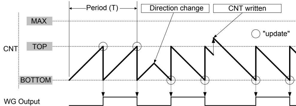
Figure 20-9. Frequency Waveform Generation
