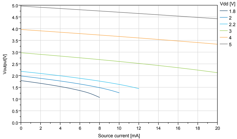
Figure 35-27. IO Pin Output Voltage vs. Source Current (T=25°C)
