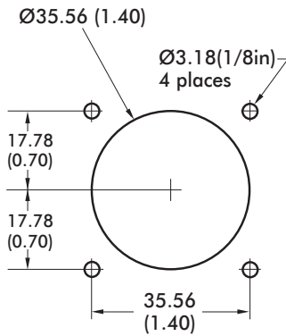
FLUSH MOUNT *
