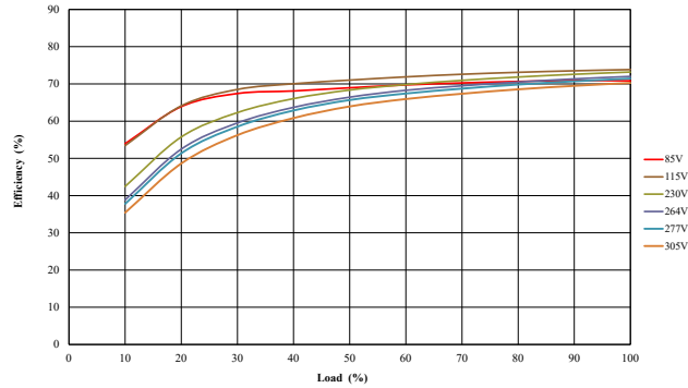
BAC1S12DC
