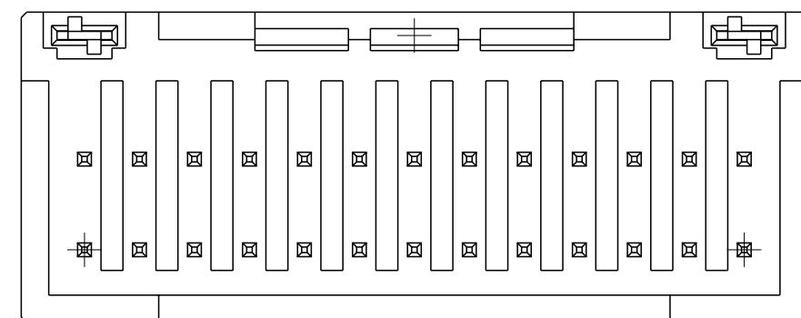
26POS(X-KEY): I-1827872-3
