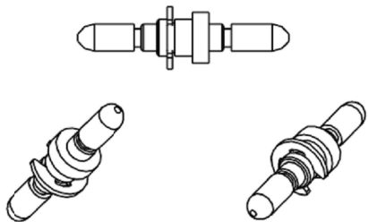
1-2308298-3 (MOUNTED) (1:1)
