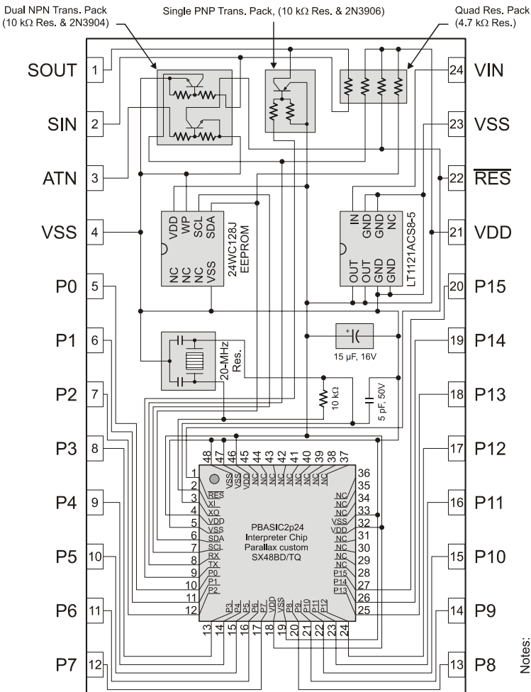
BASIC Stamp 2p24 Schematic (Rev C)
