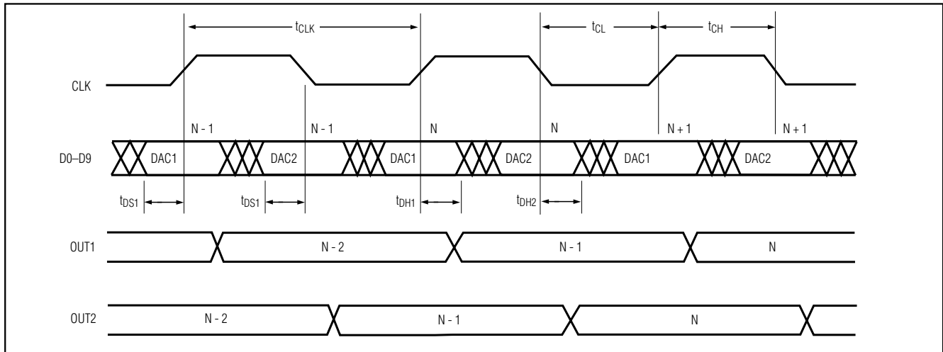
Figure 4. Timing Diagram
