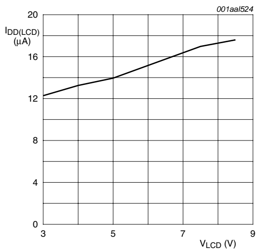
Fig 20. Typical I_{DD(LCD)} with respect to V_{LCD}
