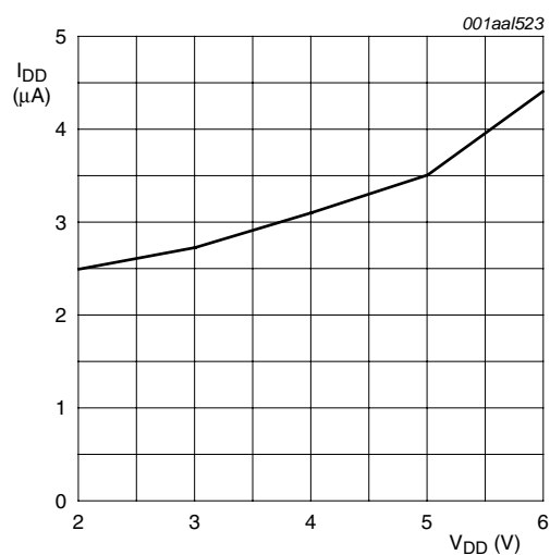
Fig 19. Typical I_{DD} with respect to V_{DD}
