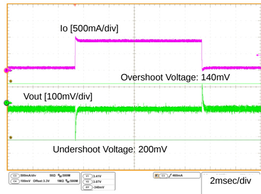
Fig.24 Load Response I_{out}: 100\text{mA} \leftrightarrow 1\text{A}
