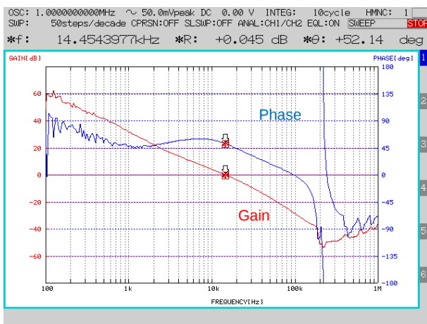
Fig.27 Frequency Response I_o = 100\text{mA}
