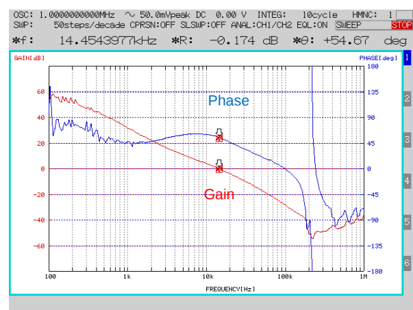
Fig.28 Frequency Response I_o = 3\text{A}
