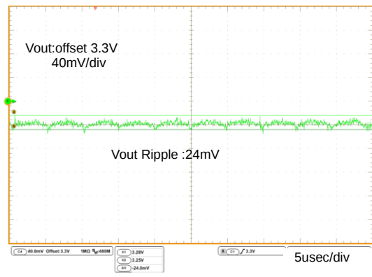
Fig.26 Lx Switching/Vout Ripple I_o = 1\text{A}
