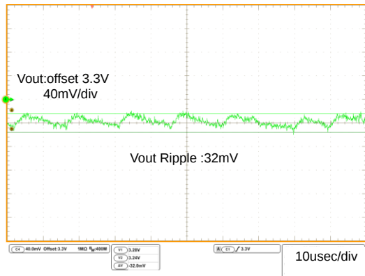
Fig.25 Lx Switching/Vout Ripple I_o = 100\text{mA}
