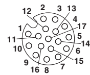
Pin assignment M12, 17-pos., female side view
