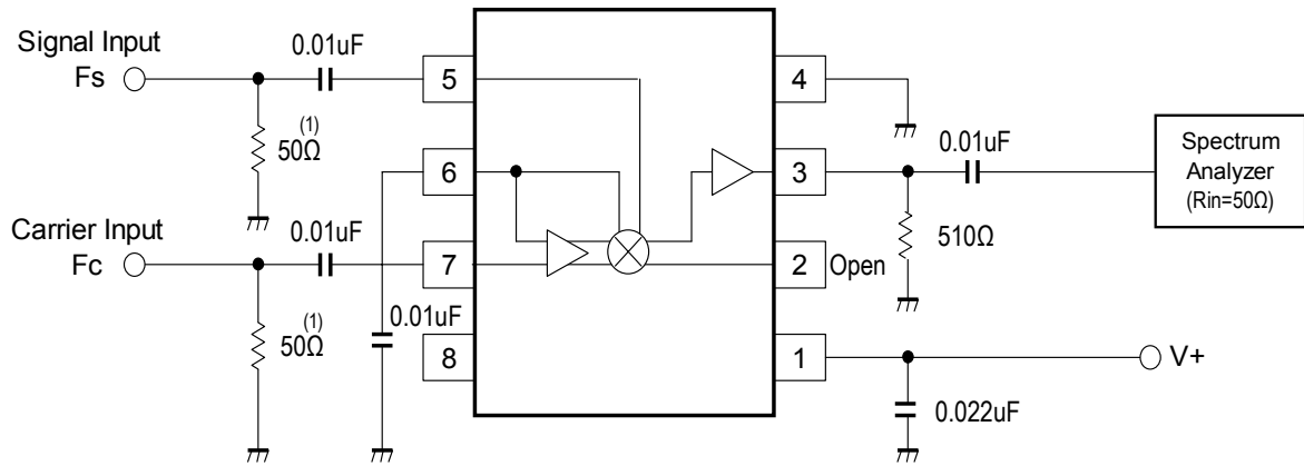
TEST CIRCUIT 1
